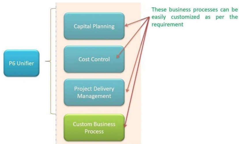
Fig 6.1. Unifier Overview
